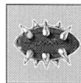
Score counter
